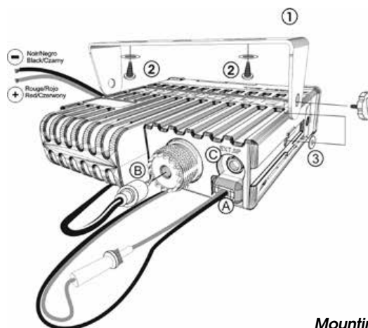
Mounting diagram
